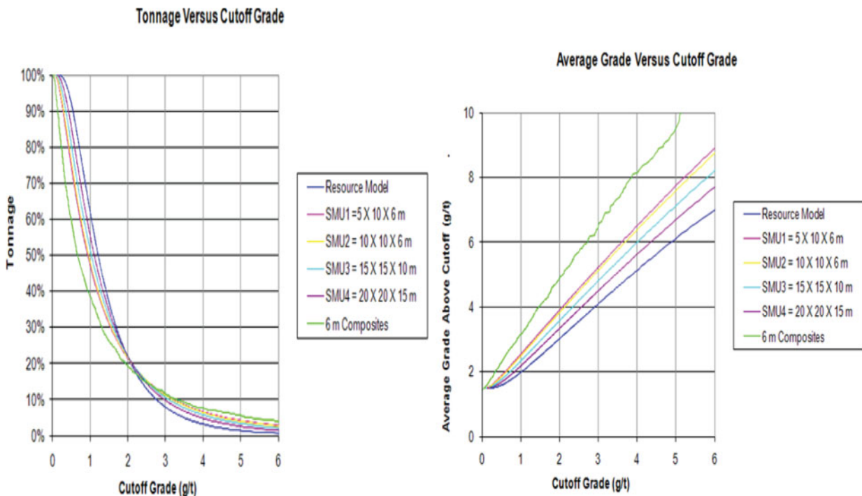
8 Grade-tonnage curves
