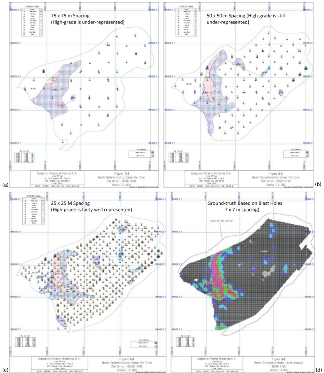
5 Zinc grade zones for three grids interpreted from experimental grids of blast holes: high grade zinc over 2.5% is red; medium grade zinc (0.25–2.5%) is blue: a 75 × 75 m spacing (high grade is under represented); b 50 × 50 m spacing (high grade is still under represented); c 25 × 25 m spacing (high grade is fairly well represented); d ground truth based on blast holes 7 × 7 m spacing
